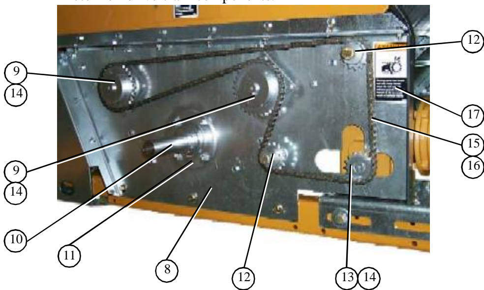
Meter roll drive train components.
